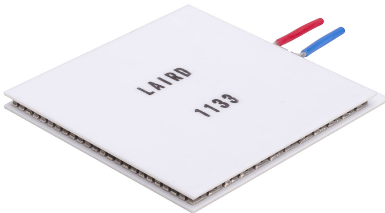
Figure 2: Laird UltraTEC Series pumps between 69 and 341 watts of heat
